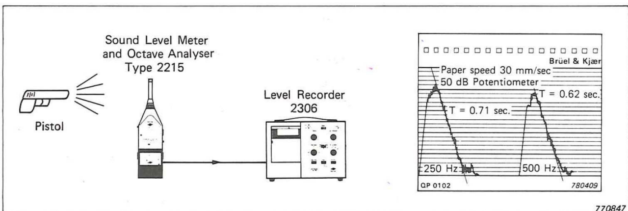
Fig. 6.1. Portable arrangement - Pistol shot method
