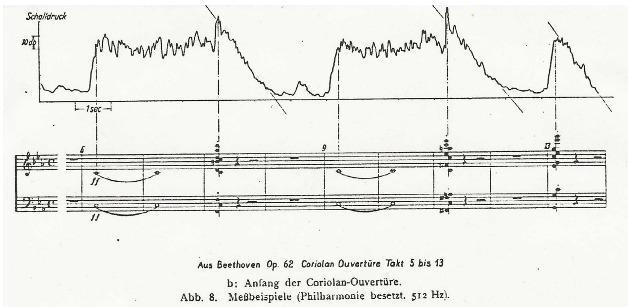
Figure 3: Decay curves in 500 Hz band measured 1934 in the old Philharmonie, Berlin, using a symphony orchestra as sound source. The music was Beethoven's Coriolanus overture, and the hall was with full audience. From Meyer & Jordan [6].
